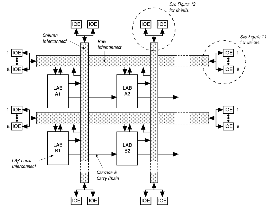
Figure 9. FLEX 8000 Device Interconnect Resources
