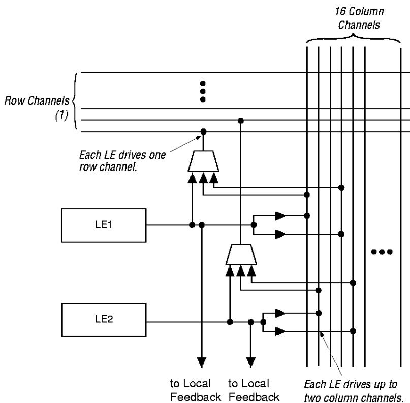
Figure 8. FLEX 8000 LAB Connections to Row & Column Interconnect
