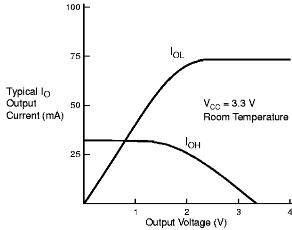
Figure 18. Output Drive Characteristics of EPF8282AV Devices
