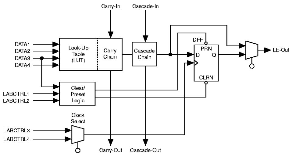
Figure 3. FLEX 8000 LE
