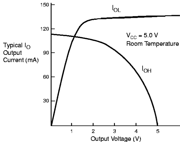
Figure 17. Output Drive Characteristics of EPF8282A Devices with 5.0-V V GGIO
