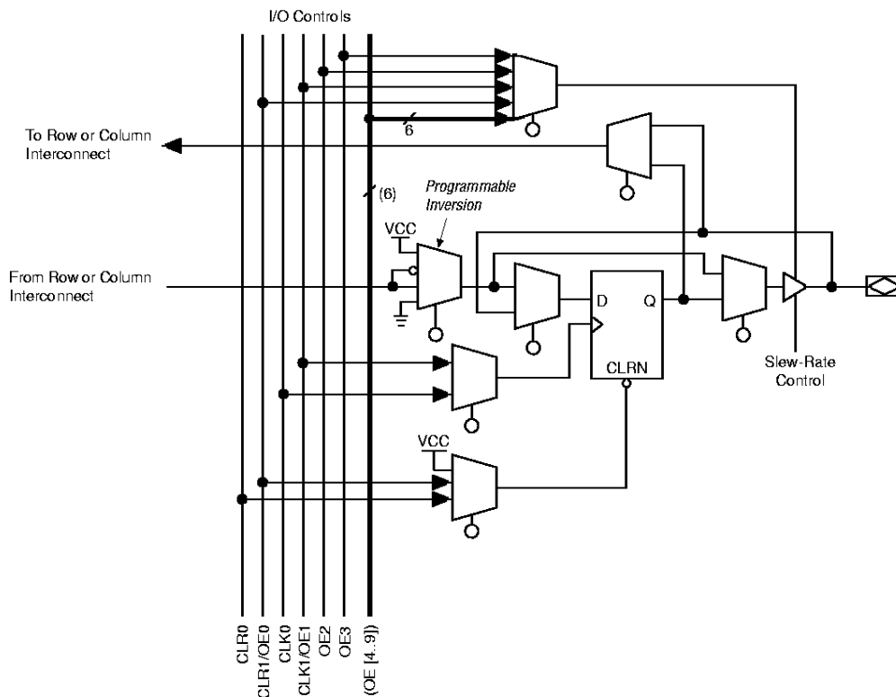
Figure 10. FLEX 8000 IOE
